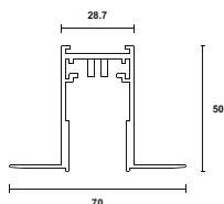
MT 003 RECESSED TRACK
