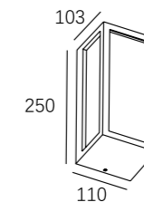
LWL-009 Watt: 18w Dimension(mm): 103x250x110 LED: E27 HOLDER Material: Die-cast Aluminium Body color: Black CRI: T IP: IP44
