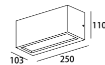
LWL-012 Watt: 18w Dimension(mm): 103x250x110 LED: E27 HOLDER Material: Die-cast Aluminium Body color: Black CRI: T IP: IP44
