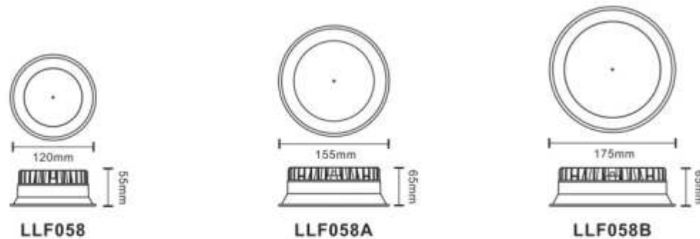
LED DEEP DOWN LIGHT SLIM BORDER SERIES
