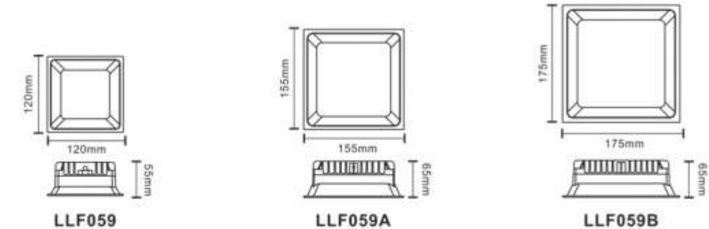
LED DEEP DOWN LIGHT SLIM BORDER SERIES
