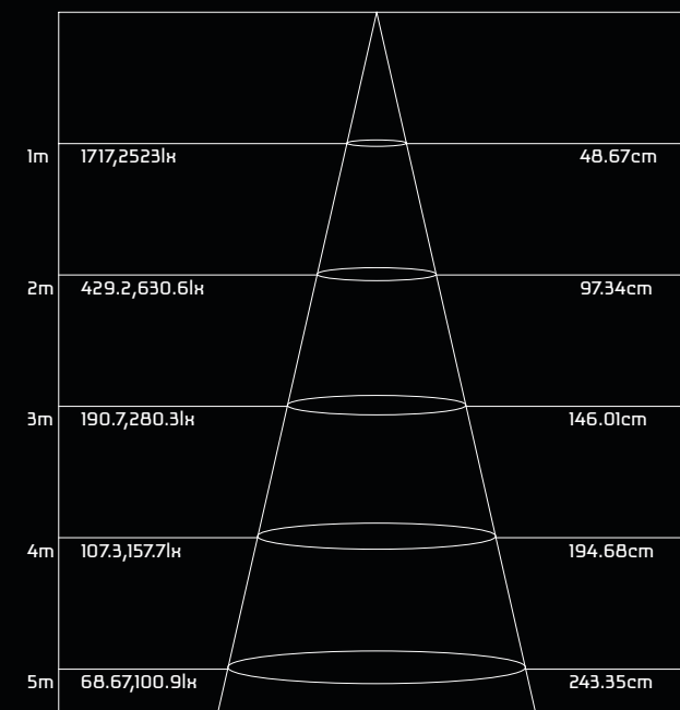
AVERAGE ILLUMINANCE AT A DISTANCE
