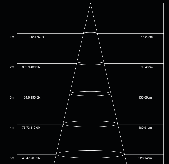
AVERAGE ILLUMINANCE AT A DISTANCE
